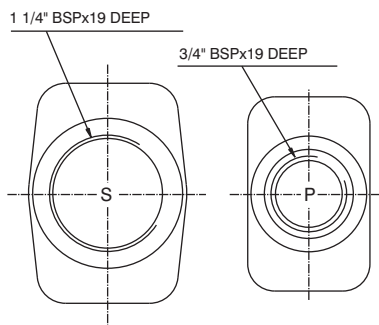
PORT CONNECTION 02
