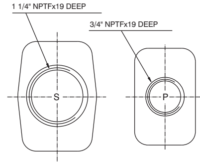
PORT CONNECTION 0X
